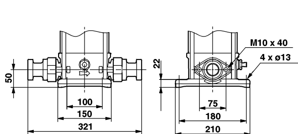
Connection to EN/DIN 11851 for CRI, CRN 1s, 1, 3 and 5
