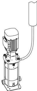
Tandem seal arrangement with a flushing-liquid supply
