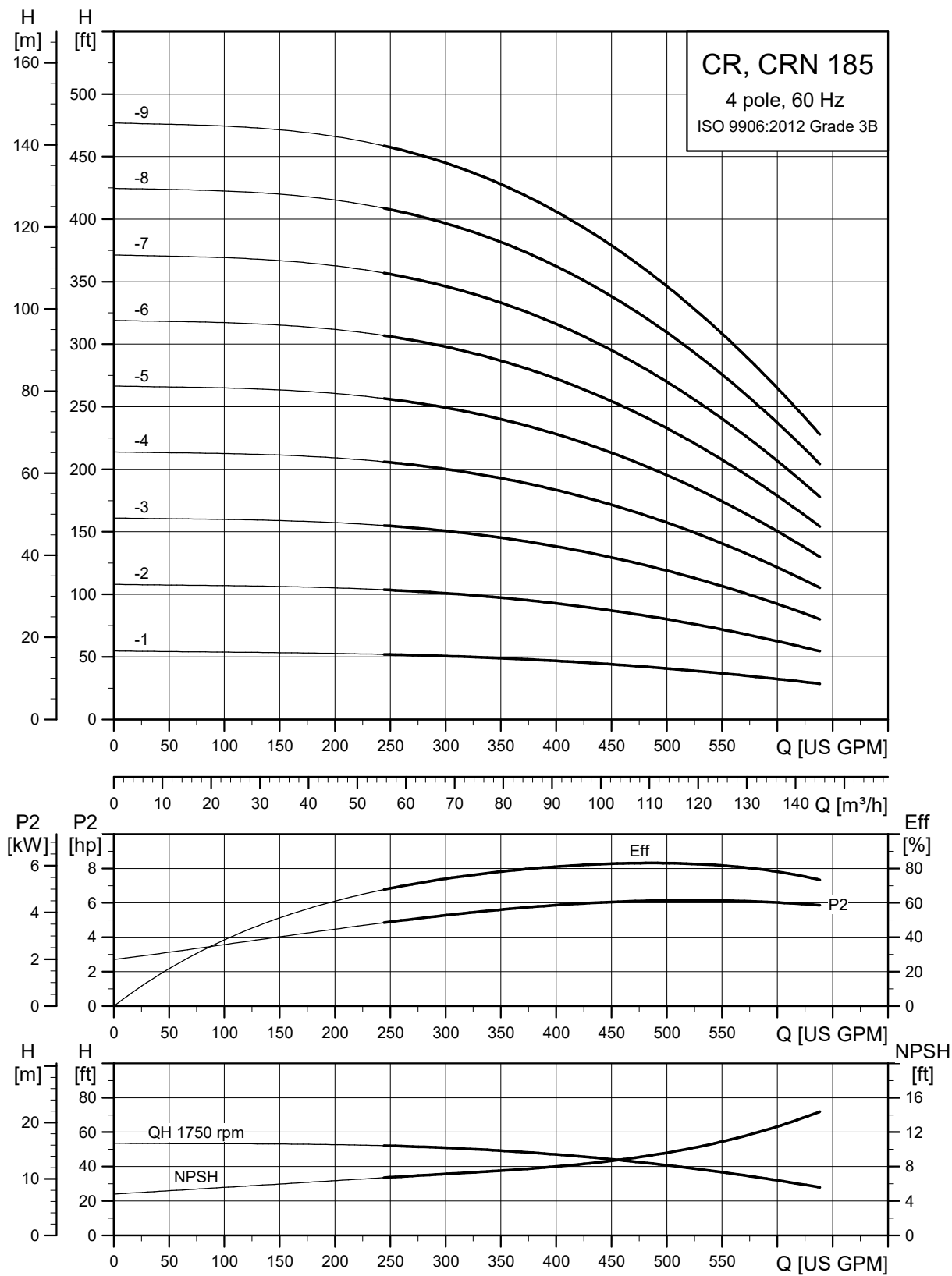
CR pumps with 4-pole motor: CR, CRN 185
