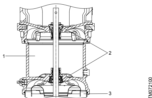
CR 95, 125 and 155 with a back-to-back seal arrangement
