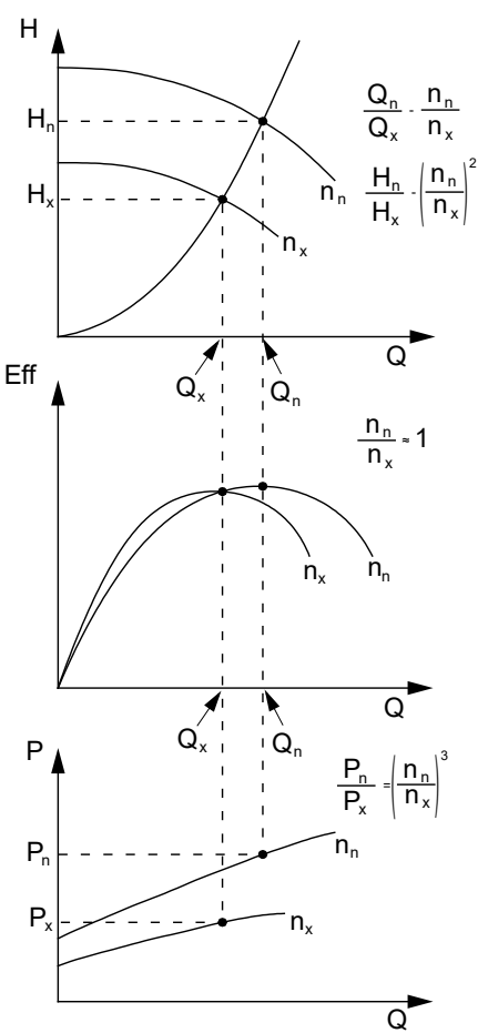
Affinity equations
