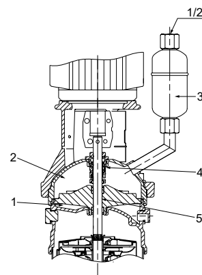
CR 10, 15 and 20 with an air-cooled top
