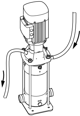
Tandem seal arrangement with flushing liquid connected to a drain
