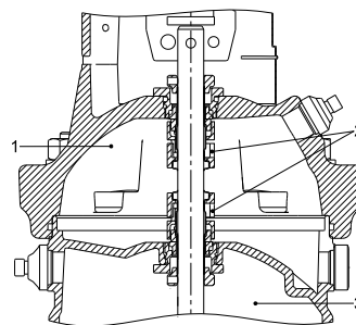
CR 10 to 20 with a back-to-back seal arrangement
