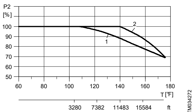
Relationship between motor output (P2) and ambient temperature (T) and altitude (ft)
