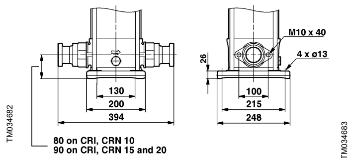
Connection to EN/DIN 11851 for CRI, CRN 10, 15 and 20
