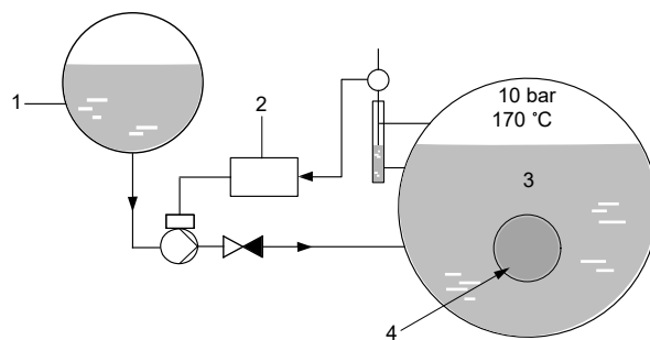
Boiler-feed application with speed-controlled pump
