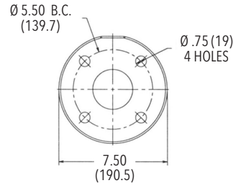
Cast Iron 2 1/2" Class 125 F.F.
